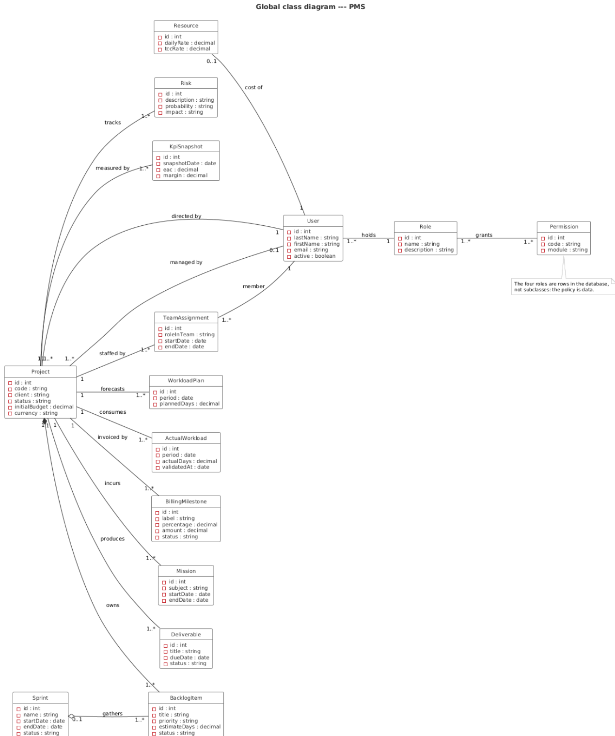
Figure 3.5: Domain model — principal classes and their associations
